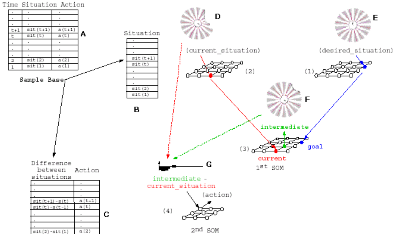
Figure 3. The lazy memory (top left) is used to build the 1 st SOM that maps the situation space, and the 2 nd SOM that maps the difference between sensory inputs vs. the action. The samples of the two learning bases have been obtained using a random action selection policy for the robot. The behavior is generated through the following process: (1) Find the neuron corresponding to the desired goal situation. (2) Find the neuron corresponding to the current situation. (3) Find a neighbor neuron (of the current situation neuron) closer to the “goal” neuron which will represent the intermediate situation to achieve. (4) Probe the 2 nd SOM with the sensory variation between the intermediate situation and the current situation to get the action that must be carried out. (A) is the sample base, (B) is the learning base of the 1 st SOM, (C) is the learning base of the 2 nd SOM, (D) is the current situation with an obstacle on the left, (E) is the goal situation with no obstacle in view, (F) is the intermediate situation to achieve, (G) is the difference between situations (F – D).
