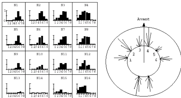
Figure 2. Left: 16 situations coded by the 16 neurons of the SOM after 100 iterations of learning. The behavior of the robot during this sampling phase is random walk. Situations are represented by a vector of 8 components. A value of 1.0 (maximum) is associated to a distance to the obstacle shorter than 2 cm. A value of 0.0 is associated to an absence of obstacle (or an obstacle at least 5 cm away). For example, neuron N1 codes for an obstacle 2 cm away on the right side of the robot ; N2 codes for larger obstacle in the same direction. Similar situations are coded by neighbor neurons. Right : The position of the 8 IR-sensors on the robot body.
