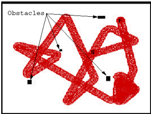
Figure 5. Obstacle avoidance behavior generated by a Nomad 200 (mobile robot) using its sonar sensors (16). The position of the robot is indicated by a circle. The robot starts in the center of the area (S: start position) and moves towards the right (F: final position). It avoids obstacles such as wall from a greater distance than the smaller obstacles – but it does not bump into any obstacle. The SOMs use the knowledge gathered by a random exploration of – only – 100 moves. The goal is defined as a perceived free-of-obstacle sensory situation. Both SOMs use 16 neurons and a neighborhood of 4.
