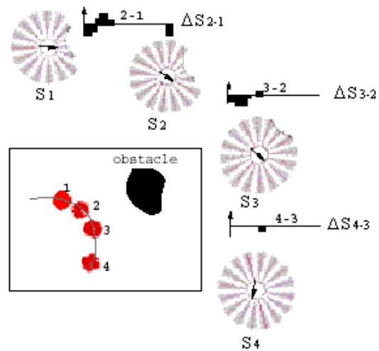
Figure 4. Example of an obstacle avoidance sequence of situations. In the box (bottom left), the successive positions of the robot and the obstacle are shown. The values of the 16-sensor sonar ring of the Nomad 200 are displayed. Also, the histograms show the sensory differences between two neighboring situations. These differences are the inputs for probing the second SOM to retrieve the actions.
